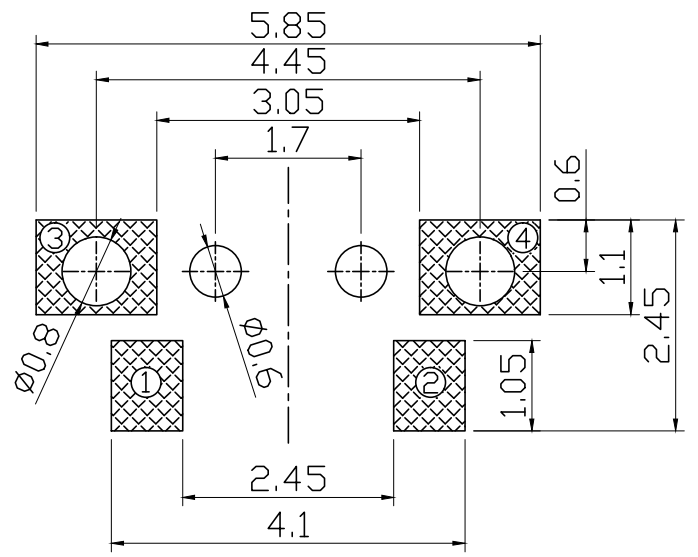
Reference P.C.B. Layout
